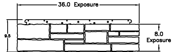
FIGURE 7 - UNIVERSAL CORNER (UN-CUT)
