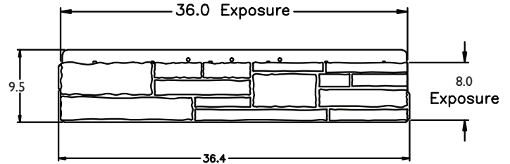
FIGURE 5 - FLAT PANEL
