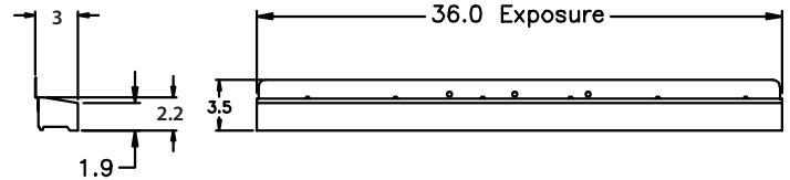
FIGURE 6 - WAINSCOT CAP
