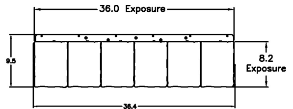
FIGURE 8 - TRIM PANEL
